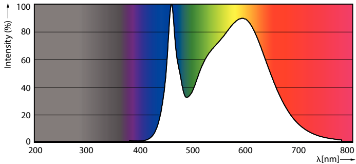
LEDlinear CorePro 7,2W R7S 840-POC
