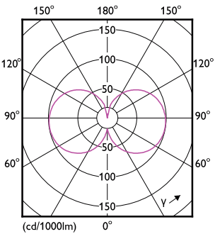
LEDlinear CorePro 7,2W R7S 840-LDD
