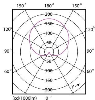
CorePro LEDbulb 100W E27 840 FR A60
