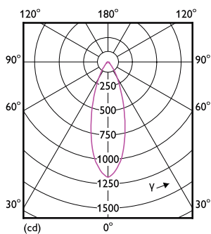
LEDspots_Corepro_7W_AR111_G53_830_40D LDD LDD
