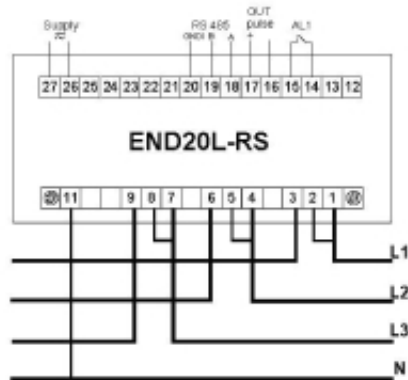
Direct connection to a three-phase network
