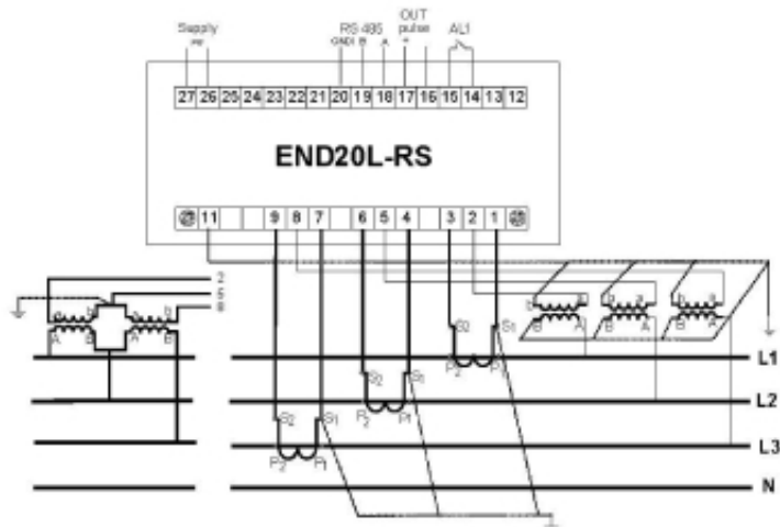
Indirect connection to a three-phase network
