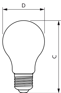
MAS LEDBulb DT7.2-75W E27 927 A60 FR G
