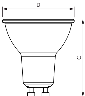
MASTER LED spot VLE D 3.7-35W GU10 927 60D
