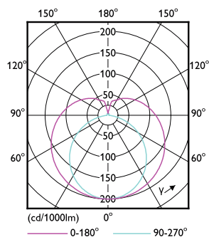
Light Distribution Diagram - MAS LEDtube 1200mm HO 26W 865 T5
