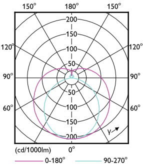
LEDtube MAS 36W G5 5600lm
