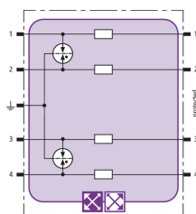
Basic circuit diagram BXT ML4 B 180
