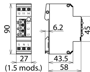
Dimension drawing DSI E 3
