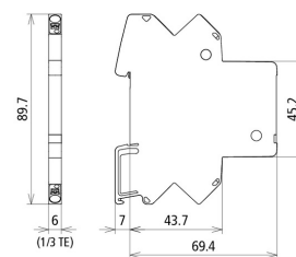
Dimension drawing BCO CL2 BE 12
