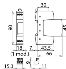
Dimension drawing DR M 2P 60 FM
