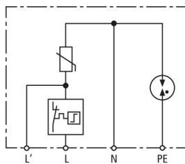
Basic circuit diagram DCOR L 2P 275 SO LTG
