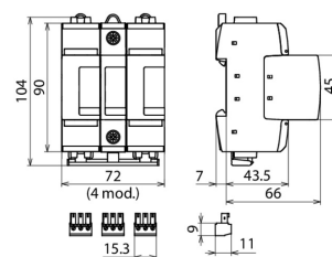
Dimension drawing DG ME DC Y 950 FM
