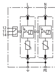
Basic circuit diagram DG M TN 150 FM
