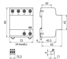
Dimension drawing DSH B TNS 255 FM
