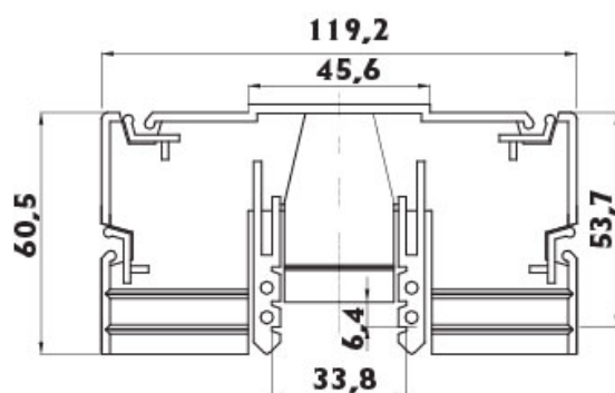
terminal plate
