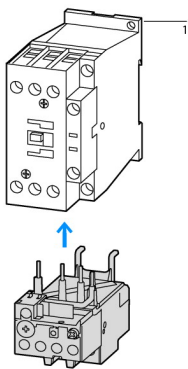
Fitted directly to the contactor
