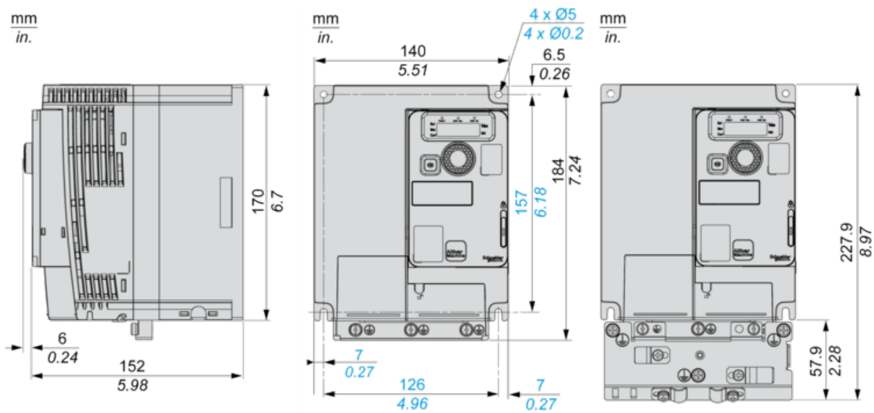
Right View, Front View and Front View with EMC Plate
